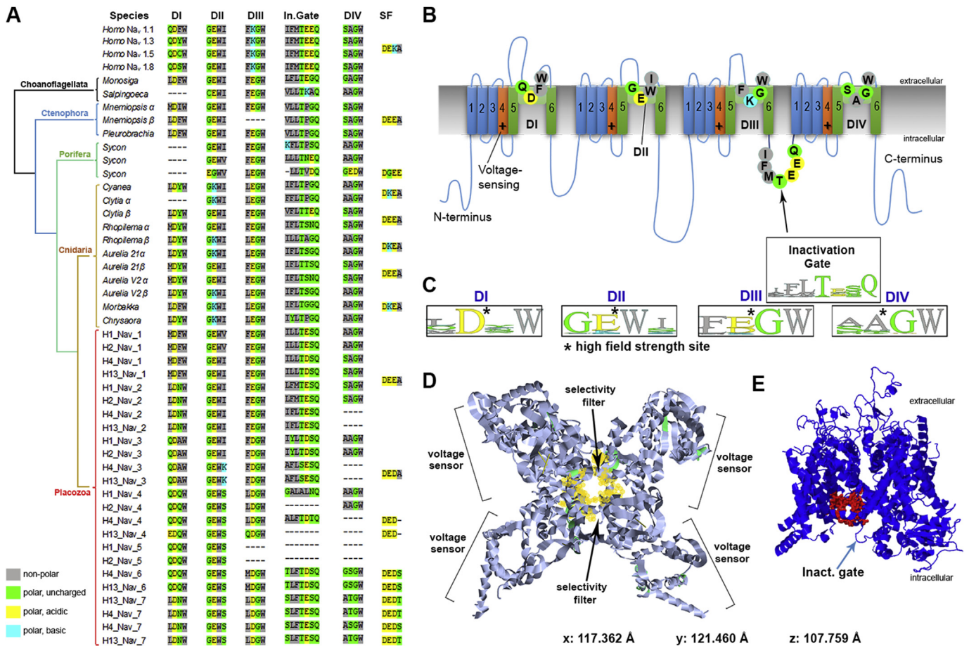
Fig. 3. Voltage-gated sodium channels ( \text{Na}_v ) in Placozoa revealed a remarkable diversity of ion selectivity pore motifs. All metazoan's \text{Na}_v have the same 4-domain organization, acquired from ancestral eukaryotes [6,31,33,35,45,51]. Here, choanoflagellates are used as the outgroup (Fig. 4). A) The table shows critical amino acids of \text{Na}_v domains (D1–D4), which contribute to pore selectivity motifs (marked as SF—Selectivity Filter [32]) and inactivation gates (In.Gate). Top four entries represent human \text{Na}_v1 ; these channels contain a critical lysine (K) in the pore region, which is responsible for sodium selectivity [6,31,32]. B) Schematic organization of a generalized sodium channel. Each of the four \text{Na}_v domain (I–IV) contains six transmembrane loops (1–6), the pore region with four key amino-acids (indicated by circles) responsible for ion selectivity (table A). The voltage sensor parts are indicated as +. A region responsible for inactivation is located between domains DIII and DIV. Selectivity pore motifs are from Homo Na v 1 subtypes [6,31,32]. C) WebLogo representation [52] of four critical amino acids forming ion selectivity filters (SF), as calculated from table A for each of the \text{Na}_v domains (DI–DIV). D–E) The reconstruction of a hypothetical 3D-structure of the \text{Na}_v -1-like channel from Trichoplax adhaerens (TriadITZ_003340). D) Top \text{Na}_v view is based on pdb ID: 6A90 modeling [53]. E) Side view of the same \text{Na}_v -1-like Trichoplax channel generated using Phyre2 modeling [54]. The structural model is close to the human \text{Na}_v1.4 type, where a 'detection' pocket is marked by red, and located close to the inactivation gate (arrow). (For interpretation of the references to color in this figure legend, the reader is referred to the Web version of this article.)
