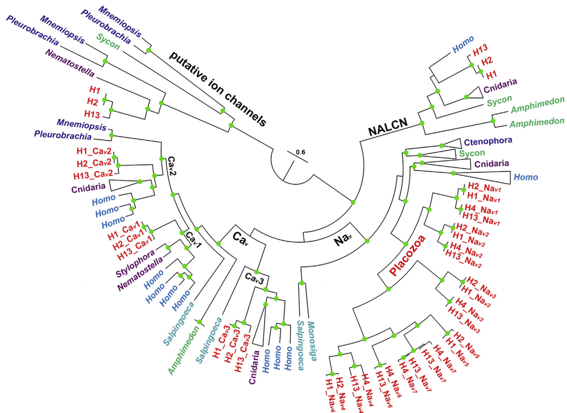
Fig. 4. The diversity and evolutionary relationships of voltage-gated sodium and calcium channels in Metazoa and two species of choanoflagellates ( Monosiga and Salpingoecia ) as outgroups. 207 protein sequences were aligned with Mafft [41]. The phylogenetic tree was reconstructed using Iqtree [42] with the VT + G4 evolutionary model. Abbreviations: Na v —voltage-gated sodium channels, Ca v —voltage-gated calcium channels, NALCN—sodium leak channels. Clade labeled “Putative ion channels” correspond to the group of sequences with no experimentally studied homologs, which mostly present in early-branching metazoan lineages. Placozoan species are denoted by mitochondrial haplotypes: H1— Trichoplax adhaerens , H2— Trichoplax sp., H13— Hoilungia hongkongensis , H4— Hoilungia sp. Selective groups of ctenophores, cnidaria, and sponges are collapsed here, but Fig. 1S (supplement) shows the expanded version of this tree. The references for each particular species, gene and/or their sequences with relevant GeneBank accession numbers are summarized in the supplementary excel Table S1.
